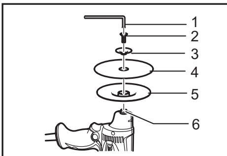
► 1. Hex wrench 2. Clamp screw 3. Countersunk washer 4. Abrasive disc 5. Plastic pad 6. Spindle
